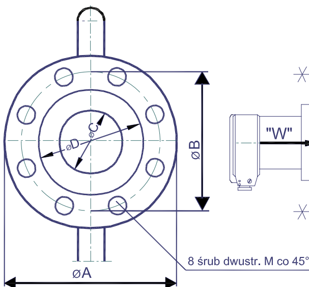
Widok "W"
